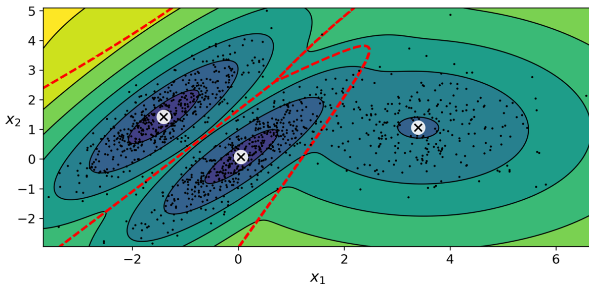
Figure 9-17. Cluster means, decision boundaries, and density contours of a trained Gaussian mixture model
